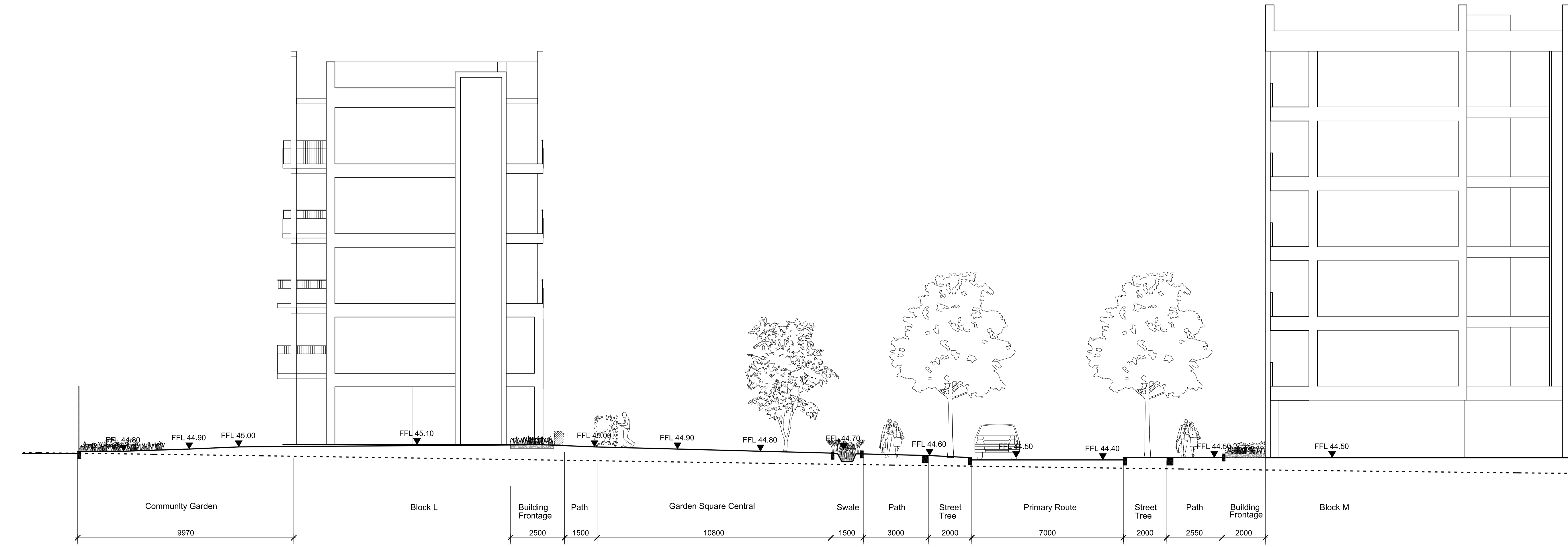
2 SECTION 20 SCALE 1:100
