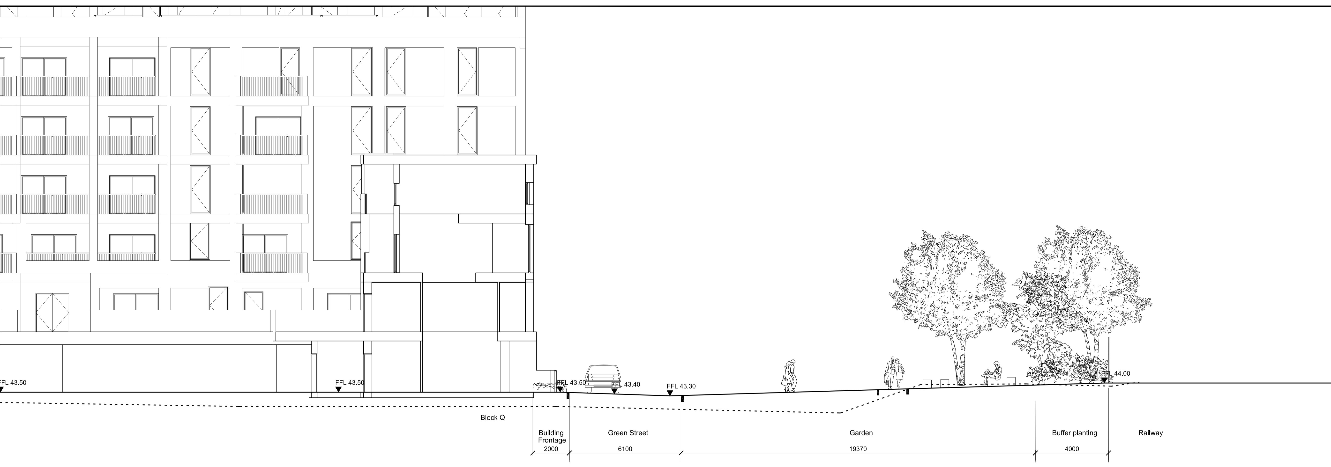
1 SECTION 13 SCALE 1:100
