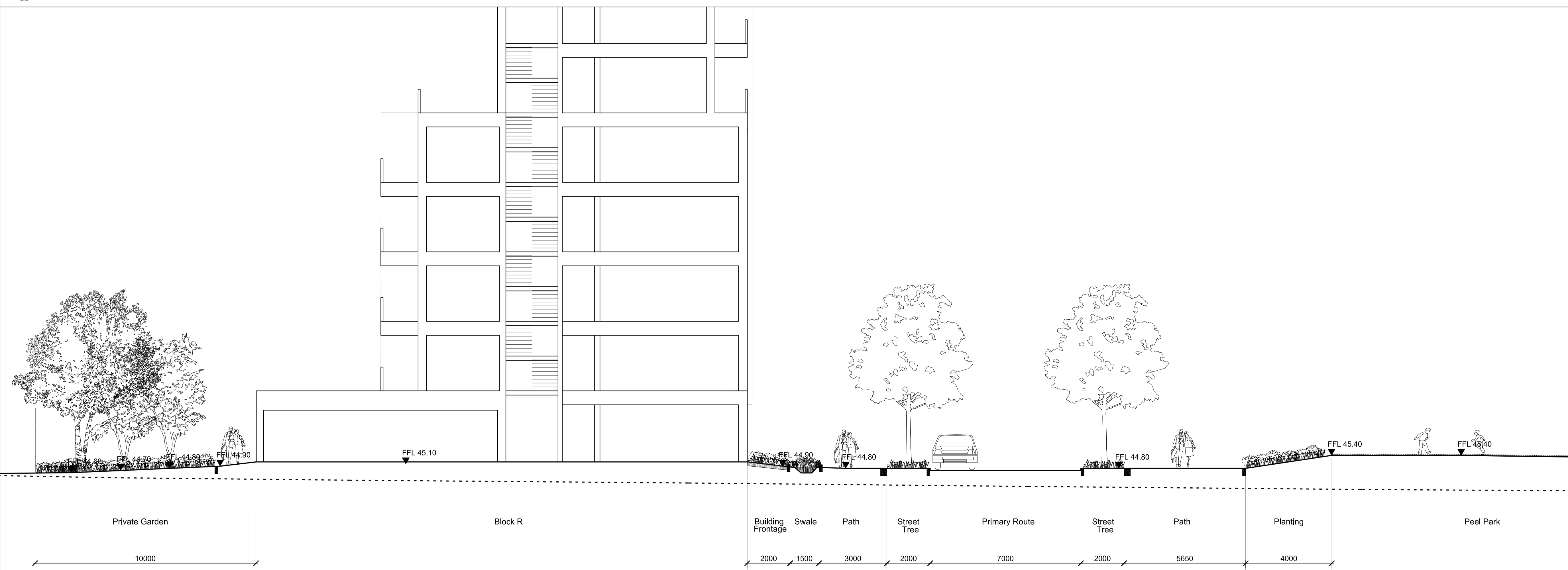
2 SECTION 10 SCALE 1:100
