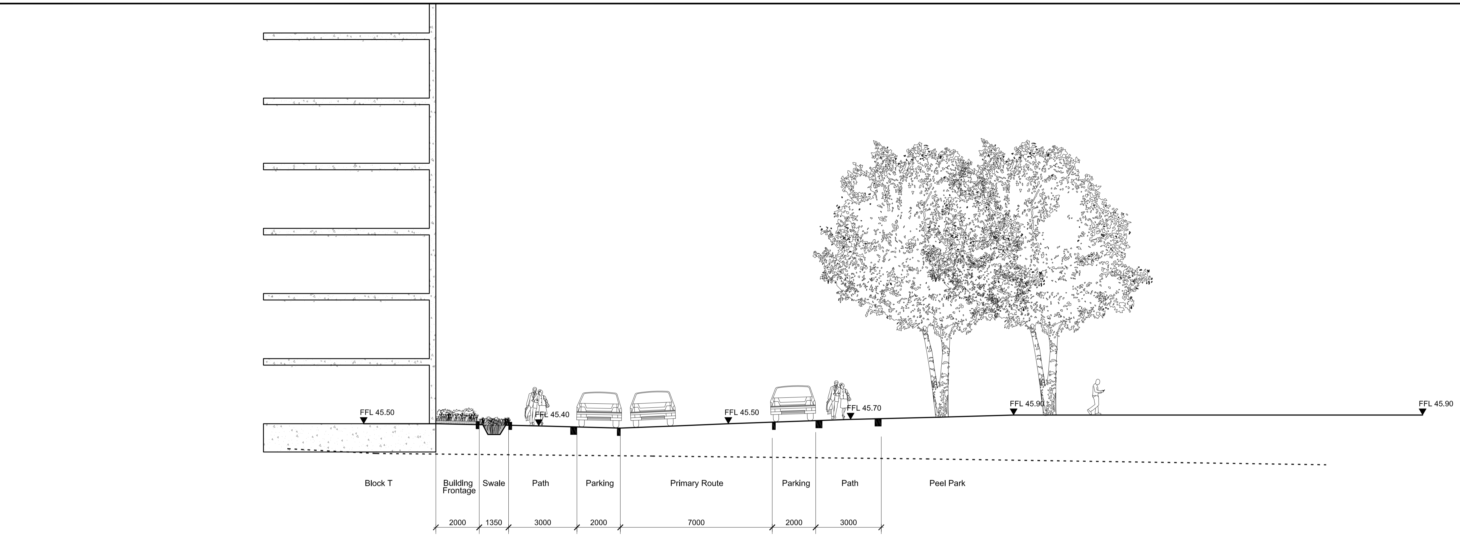
1 SECTION 07 SCALE 1:100
