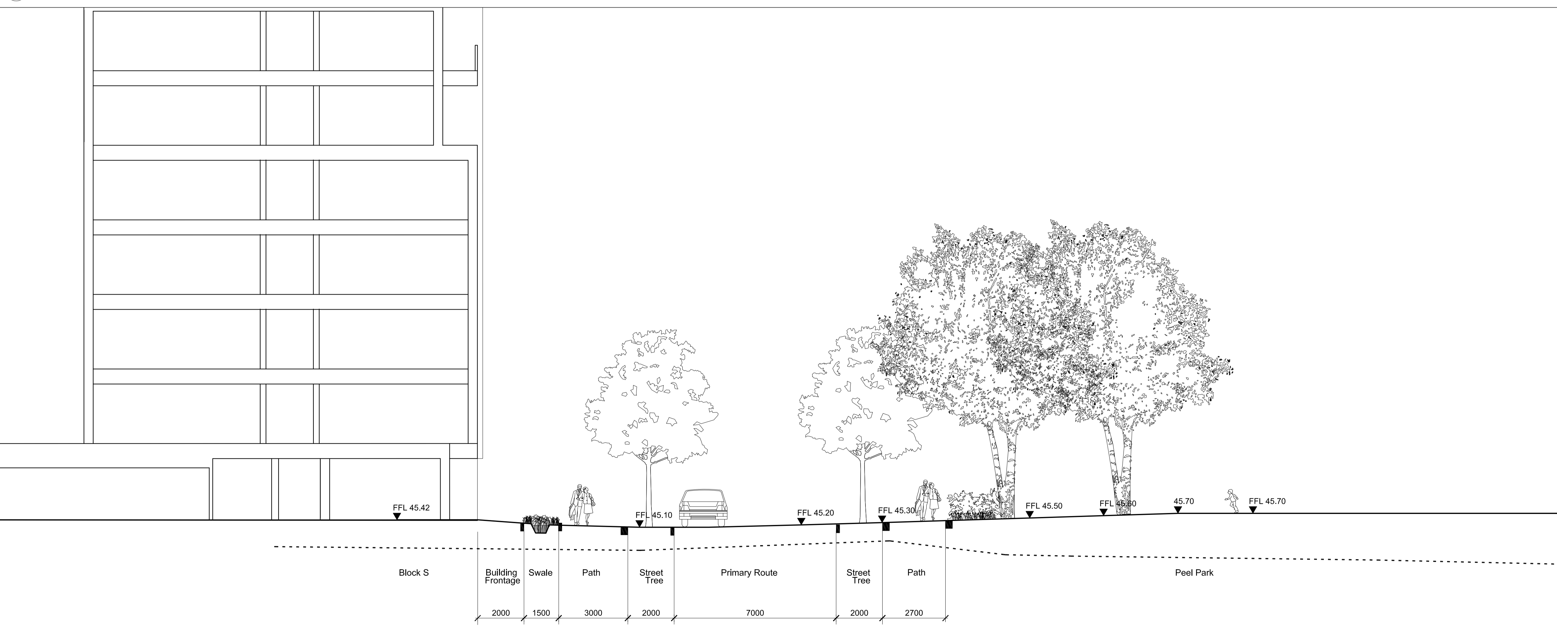
2 SECTION 08 SCALE 1:100
