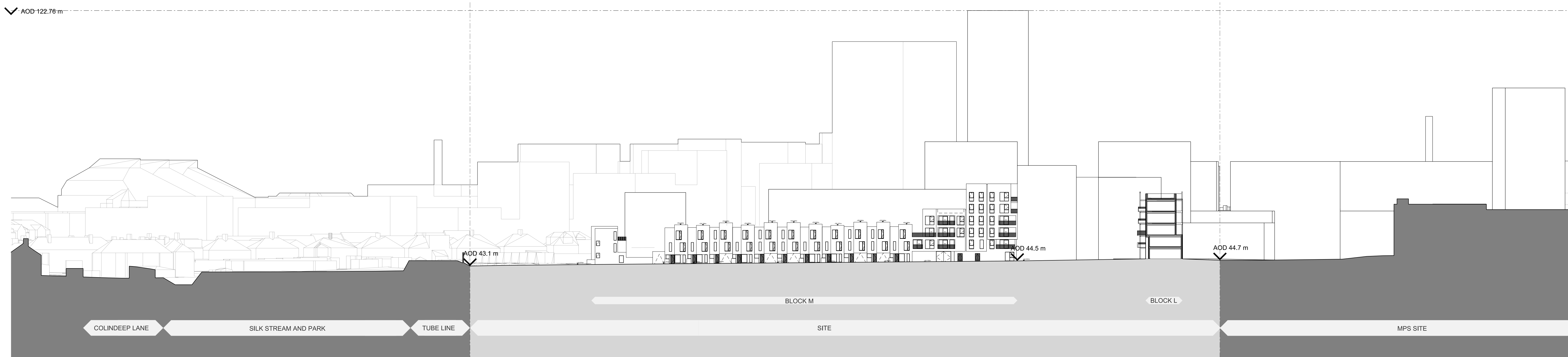
0707. 3 Section 05 - West Facing Proposal 1: 500
